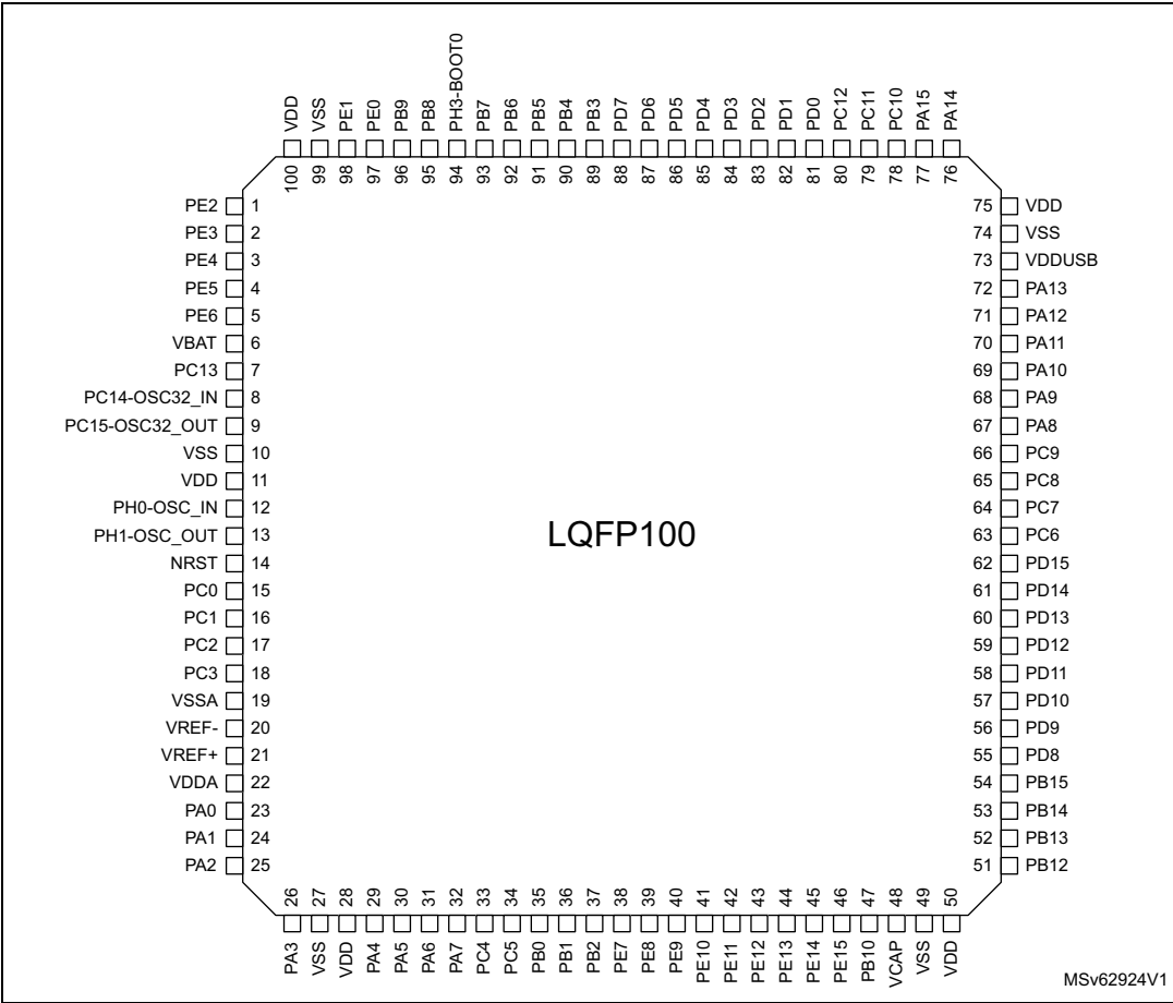
Figure 15. LQFP100 pinout
