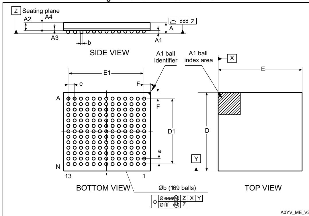
Figure 102. UFBGA169 - Outline
