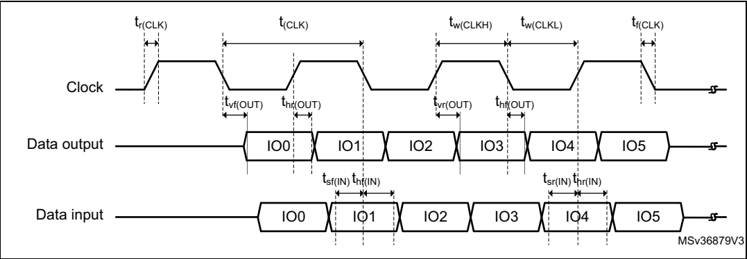
Figure 75. DDR mode
