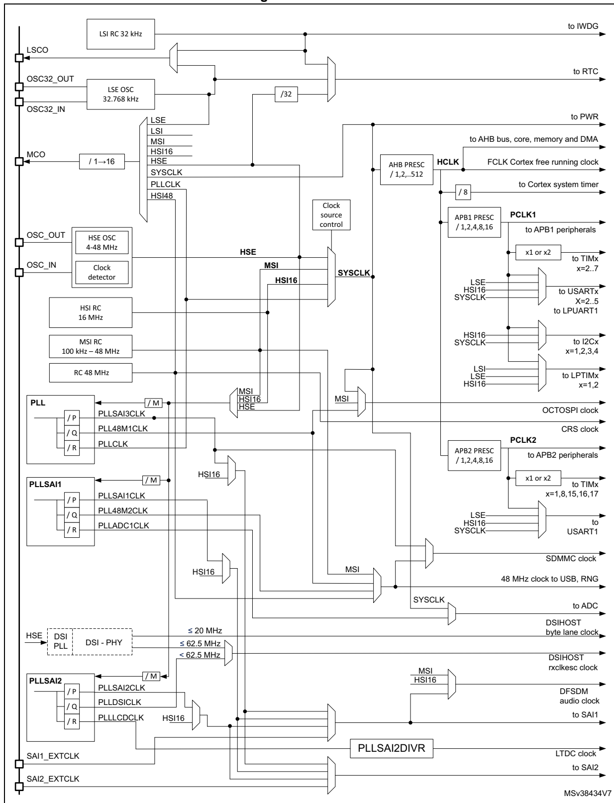
Figure 6. Clock tree
