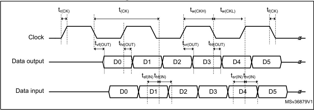
Figure 66. DDR mode
