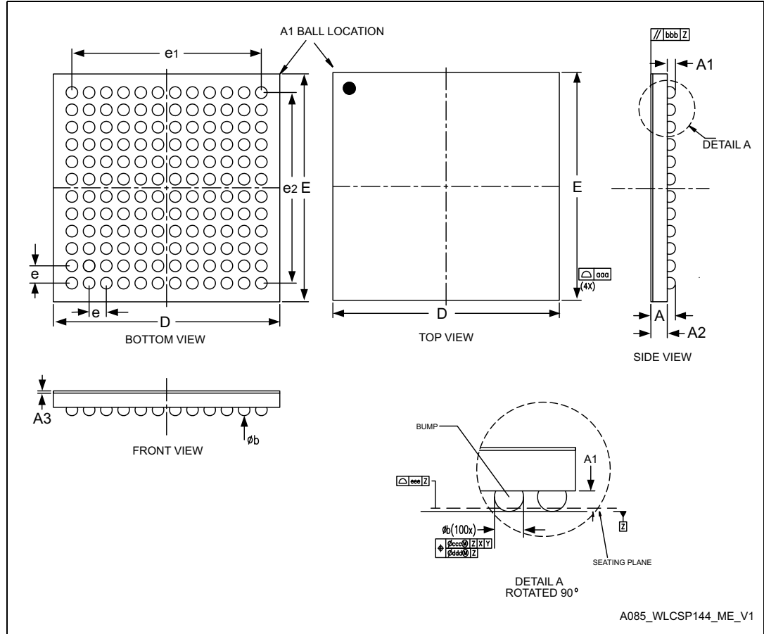
Figure 81. WLCSP144 outline
