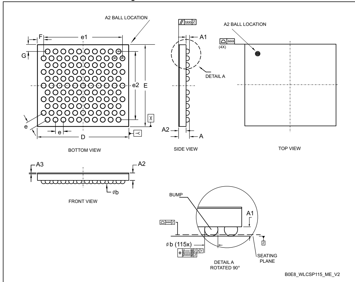
Figure 76. WLCSP115 - Outline
