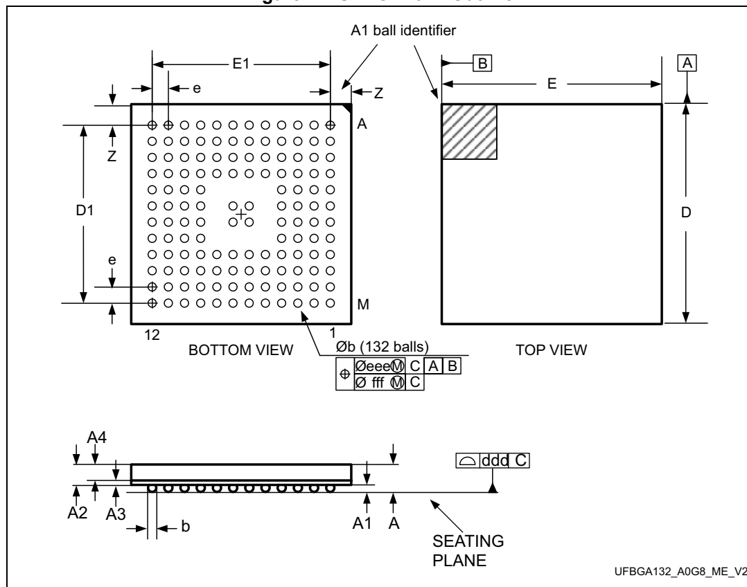
Figure 72. UFBGA132 - Outline
