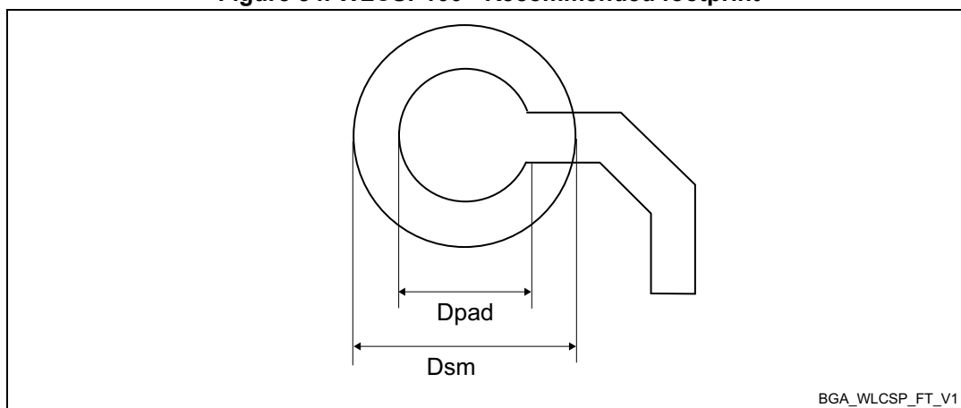
Figure 84. WLCSP100 - Recommended footprint
