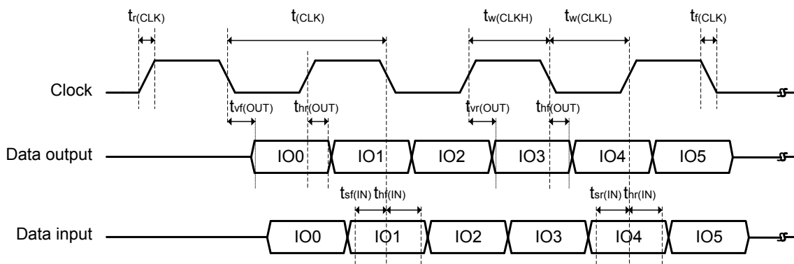
Figure 78. DDR mode
