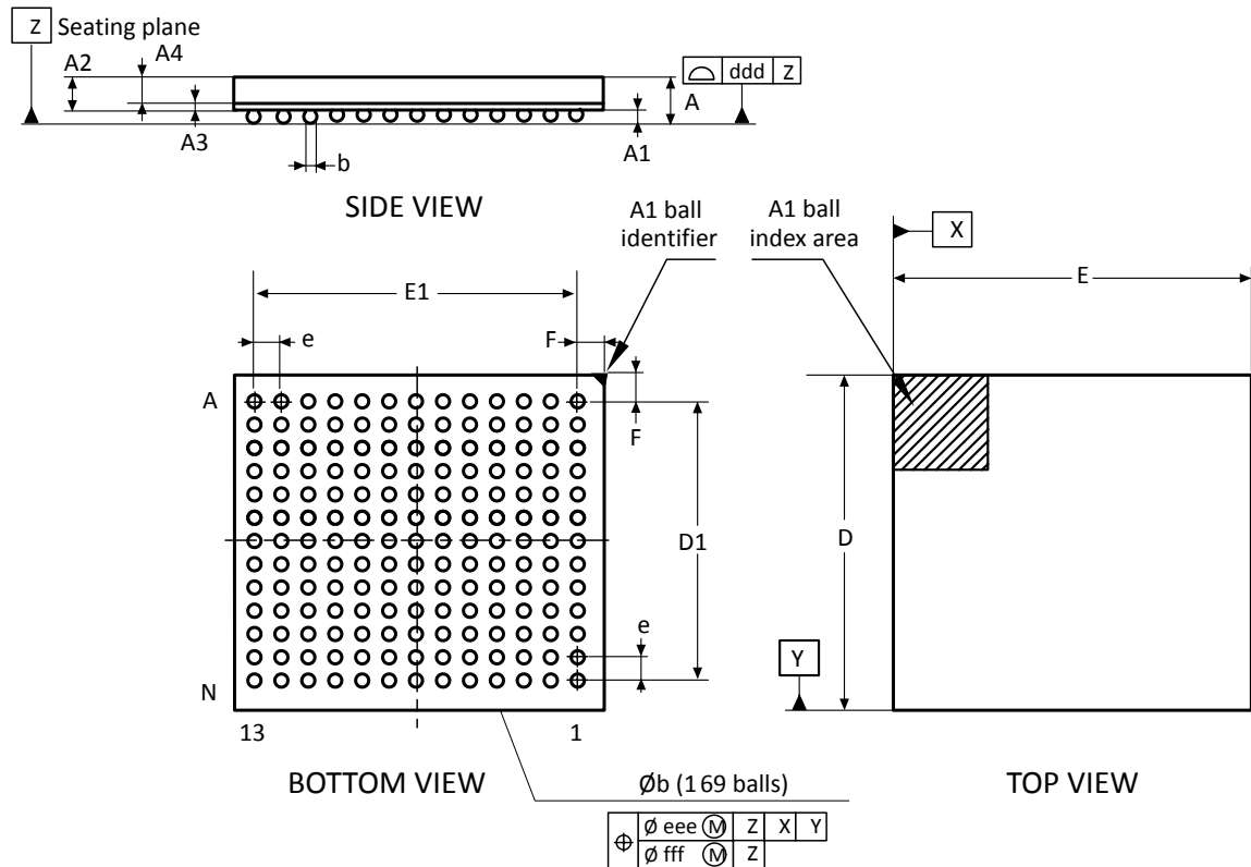
Figure 106. UFBGA169 - Outline
