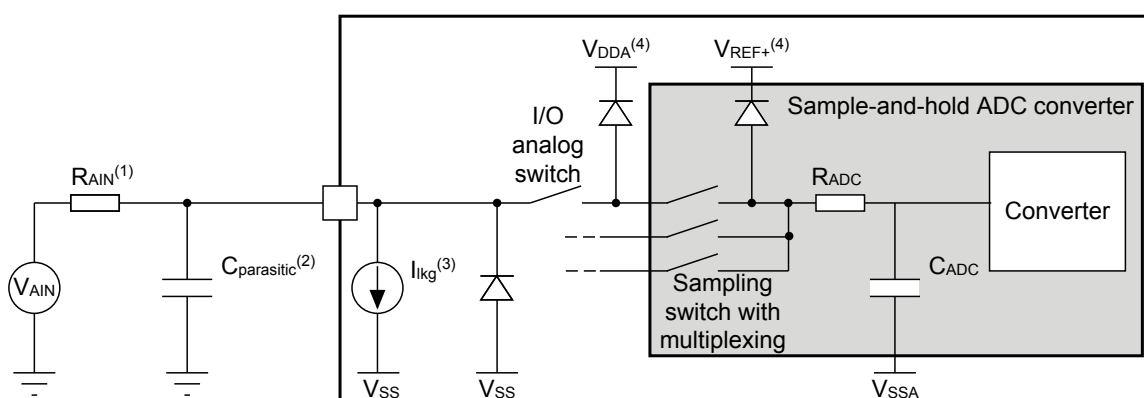
Figure 47. Typical connection diagram using the ADC with FT/TT pins featuring analog switch function
