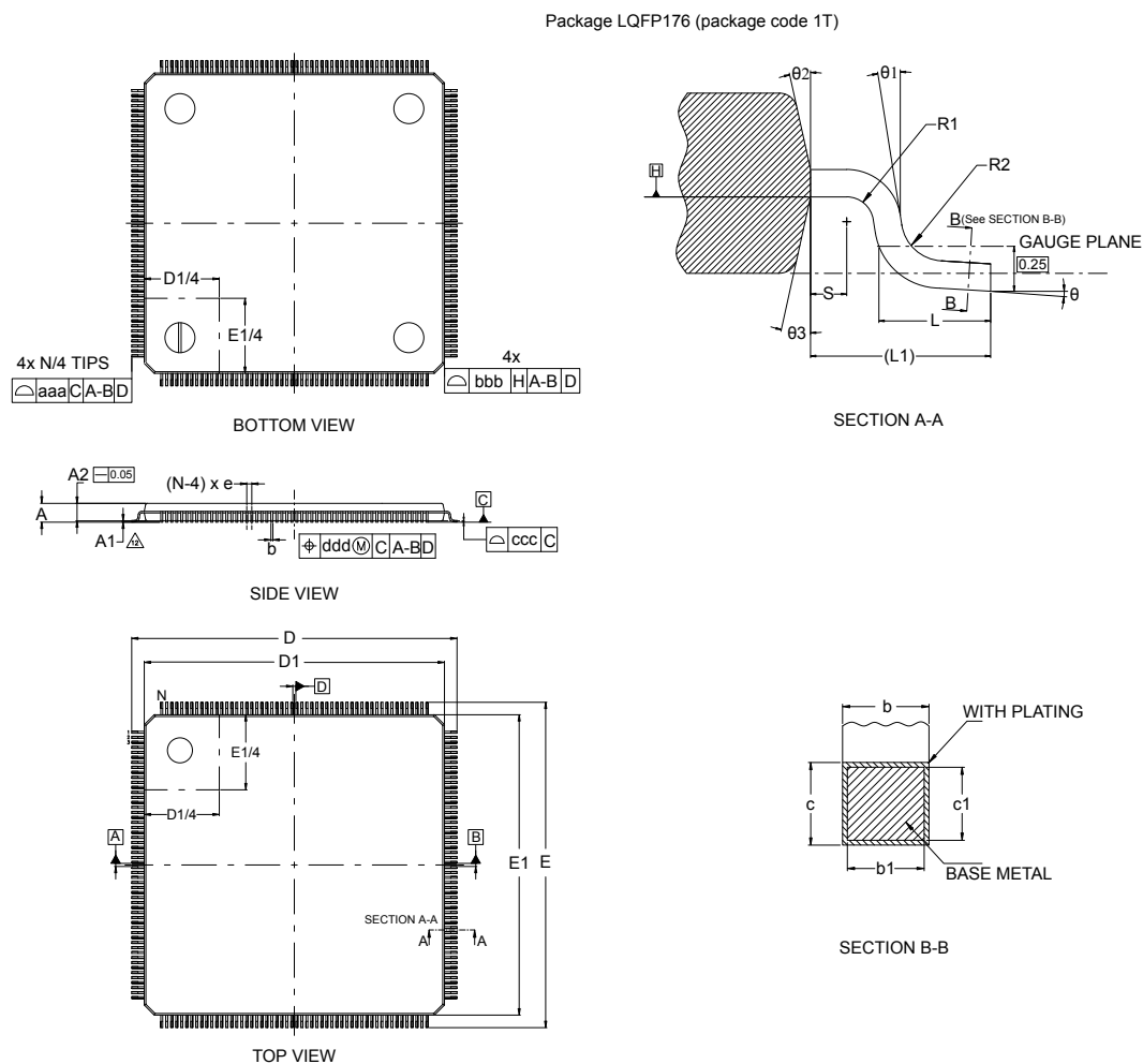
Figure 82. LQFP176 - Outline (15.)
