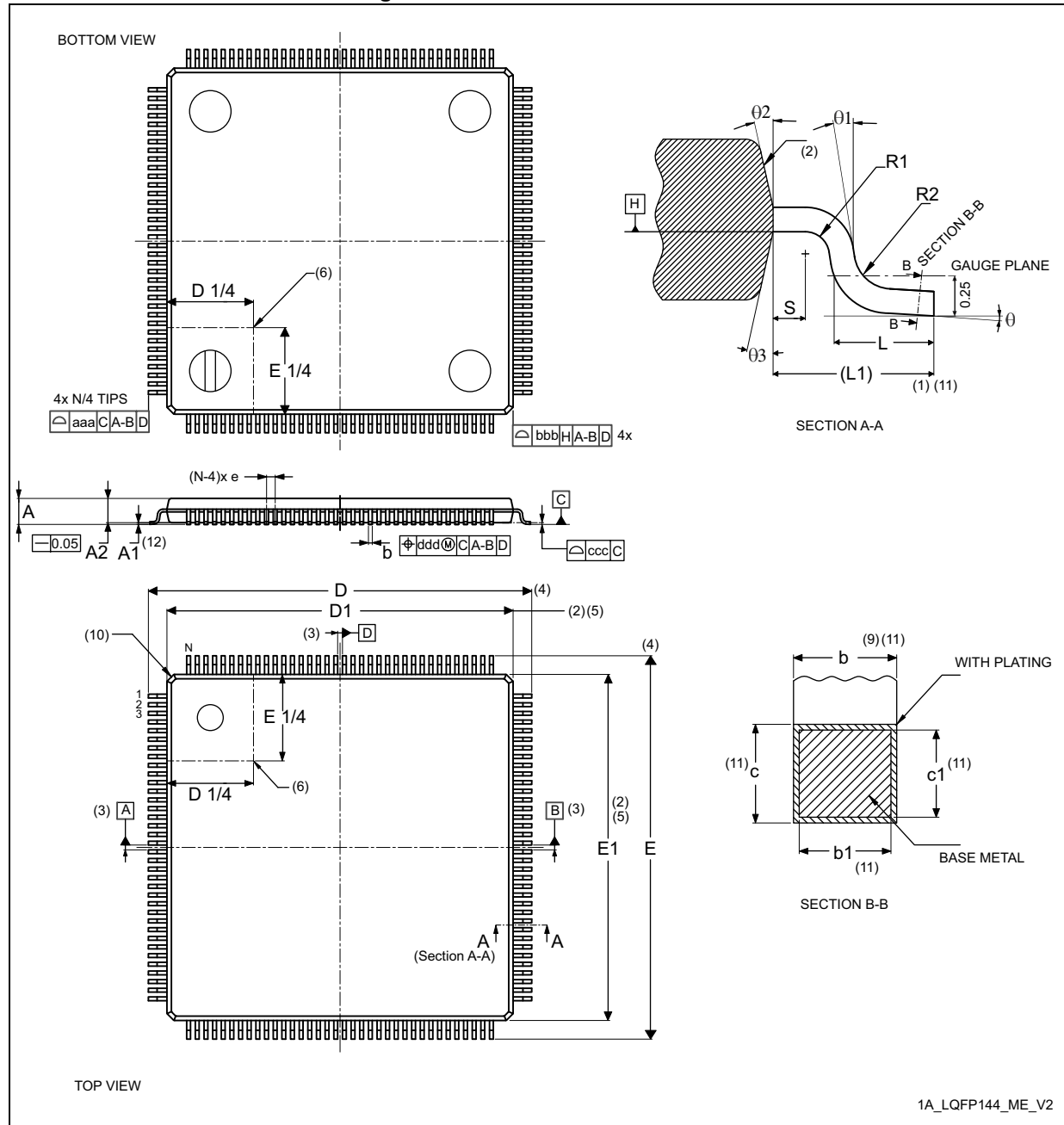
Figure 125. LQFP144 - Outline (15)
