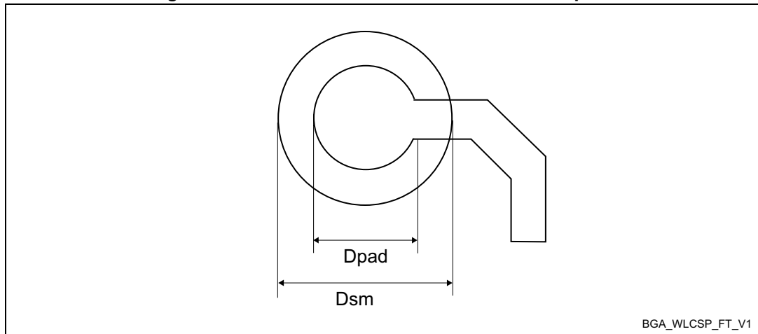
Figure 138. UFBGA176+25 - Recommended footprint
