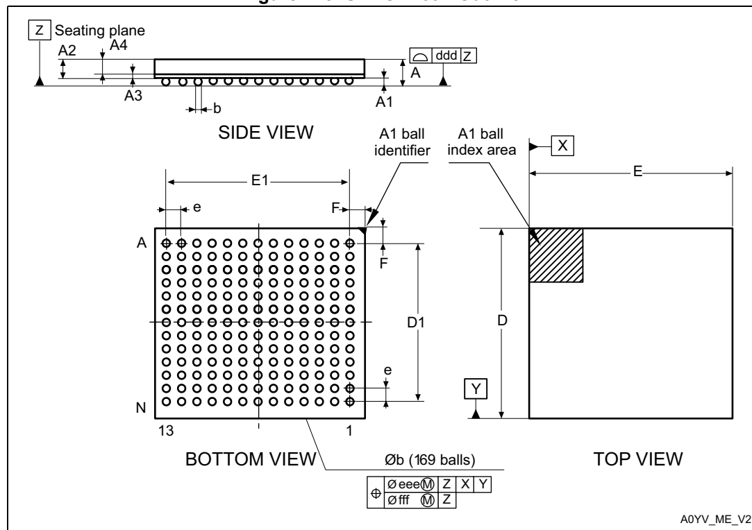
Figure 128. UFBGA169 - Outline
