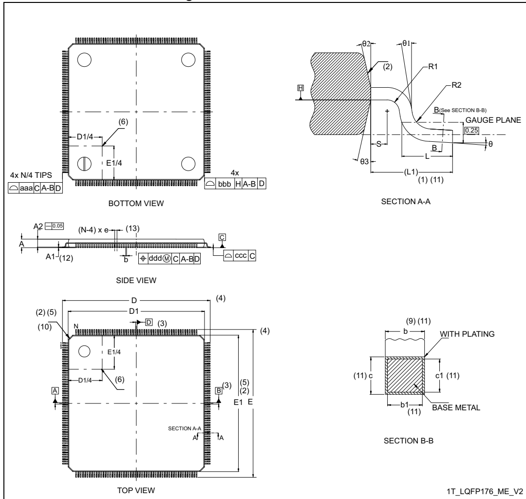
Figure 131. LQFP176 - Outline
