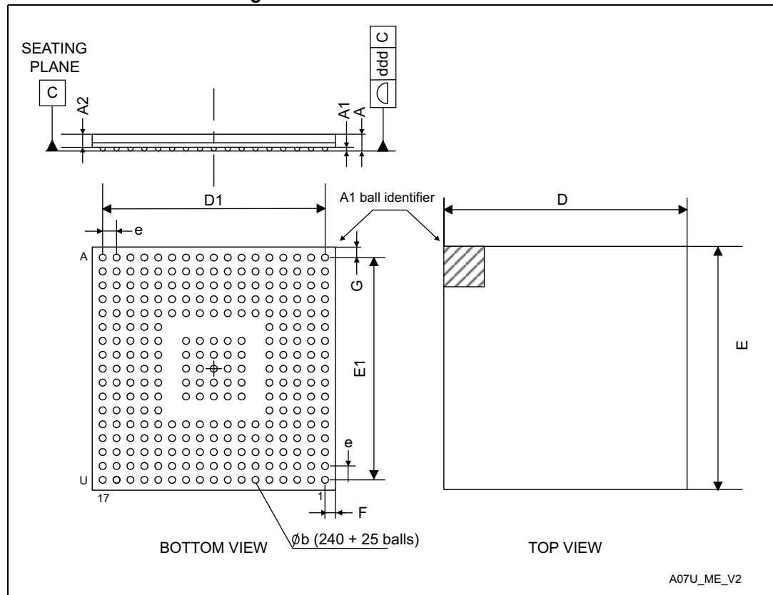
Figure 140. TFBGA240+25 - Outline
