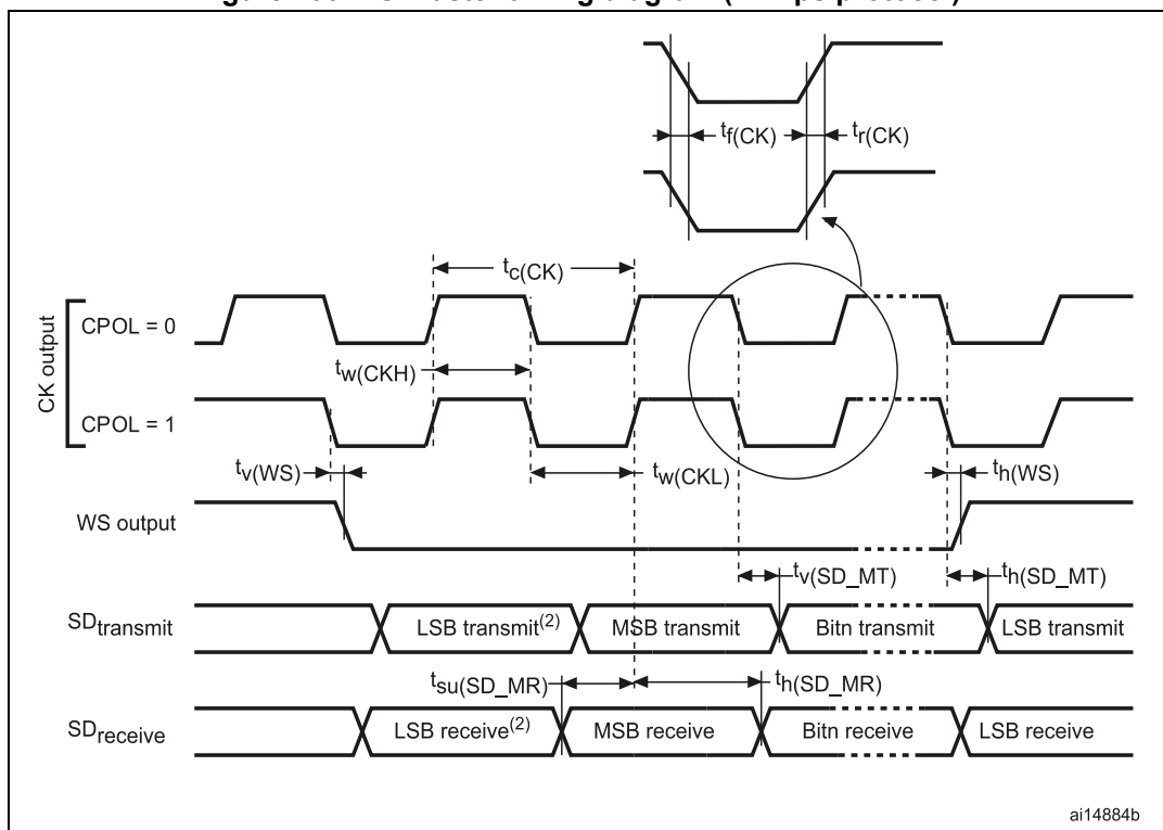
Figure 106. I 2 S master timing diagram (Philips protocol) (1)
