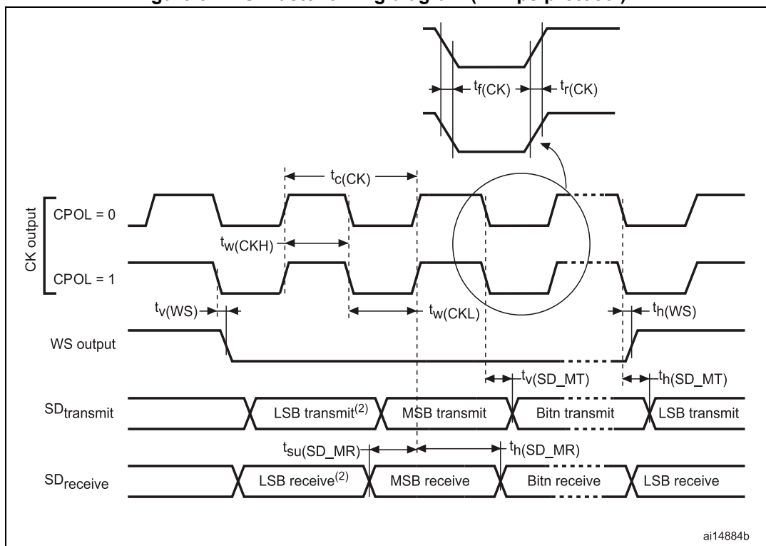
Figure 52. I 2 S master timing diagram (Philips protocol) (1)
