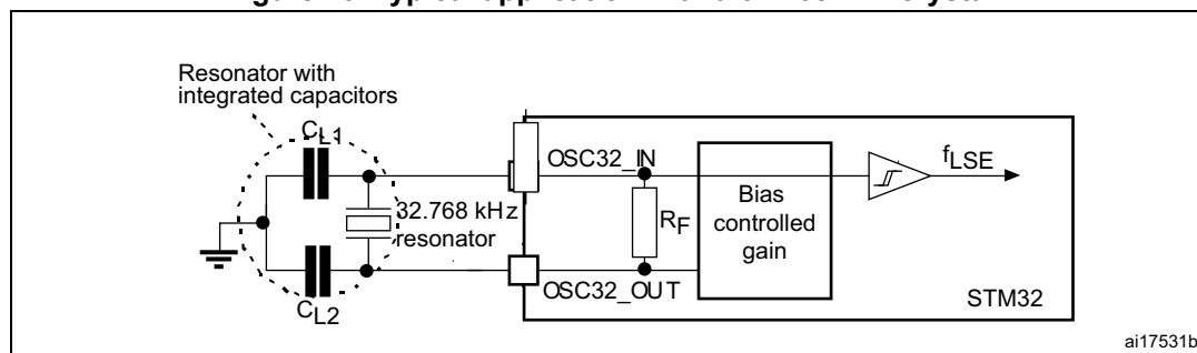
Figure 73. Typical application with a 32.768 kHz crystal
