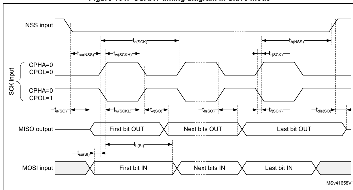
Figure 101. USART timing diagram in Slave mode
