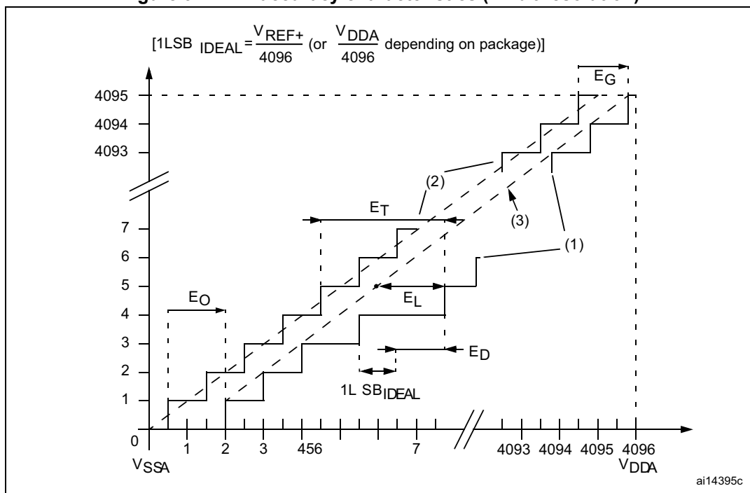
Figure 91. ADC accuracy characteristics (12-bit resolution)
