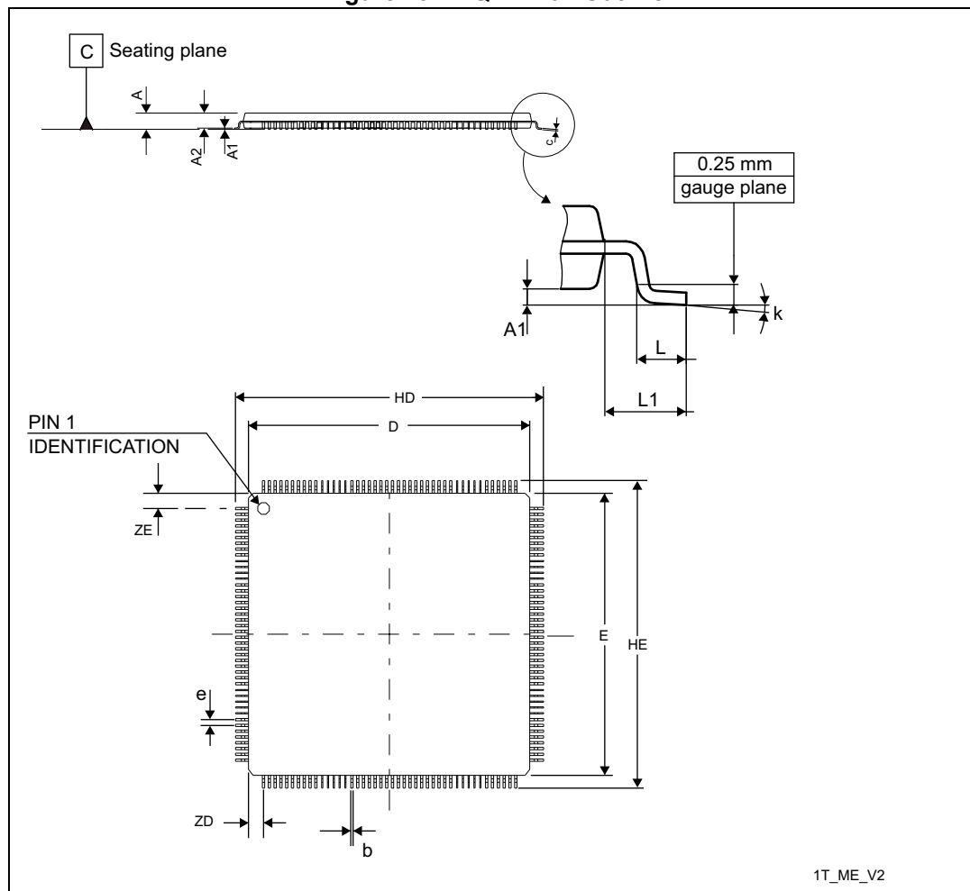
Figure 132. LQFP176 - Outline
