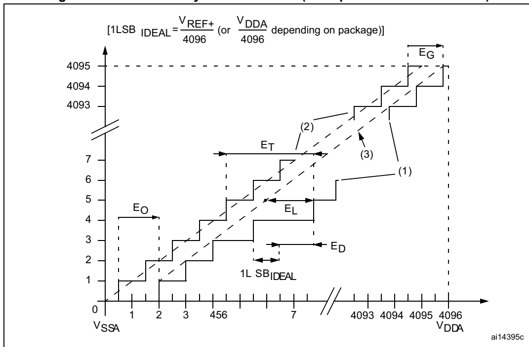
Figure 40. ADC accuracy characteristics (example for 12-bit resolution)
