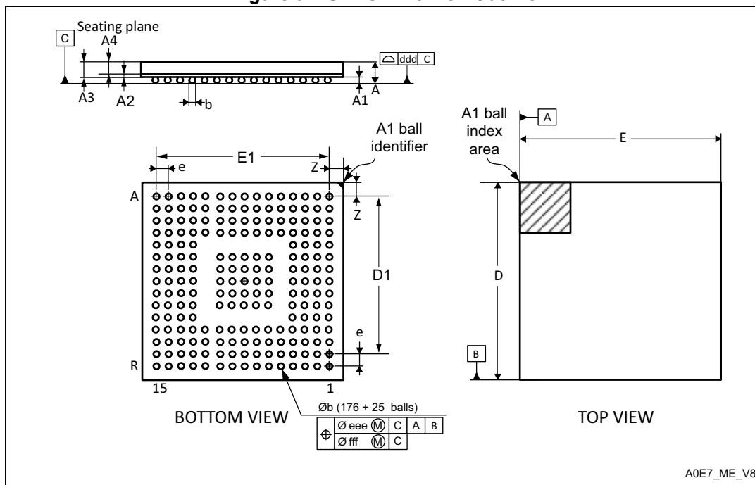
Figure 94. UFBGA176+25 - Outline
