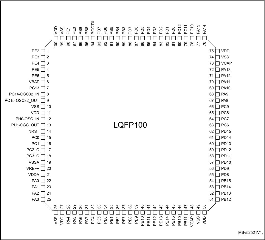
Figure 5. LQFP100 pinout (without SMPS)
