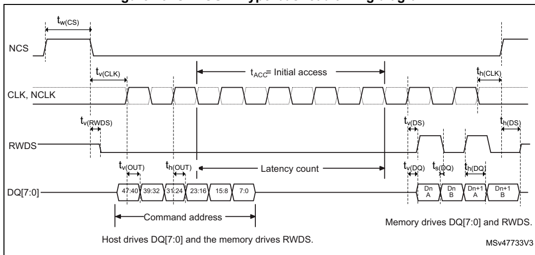
Figure 43. OCTOSPI Hyperbus read timing diagram
