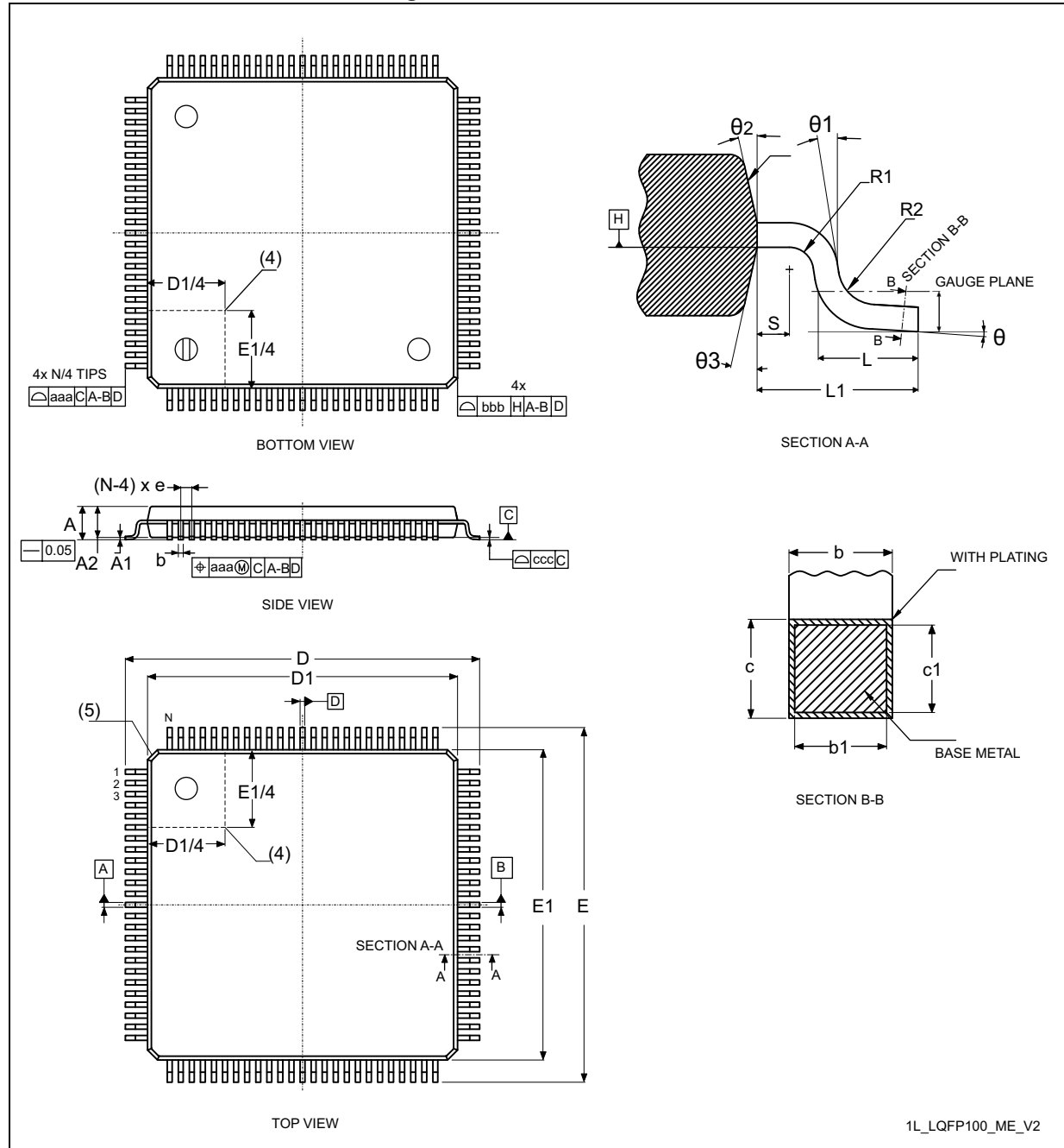
Figure 73. LQFP100- Outline
