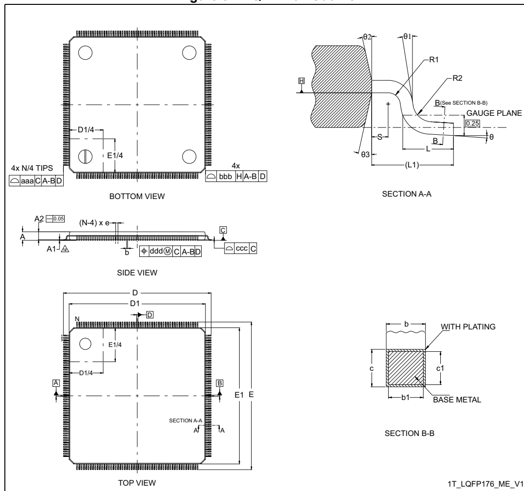
Figure 87. LQFP176 - Outline
