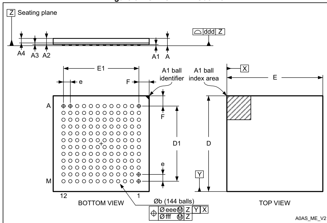
Figure 81. UFBGA144 - Outline
