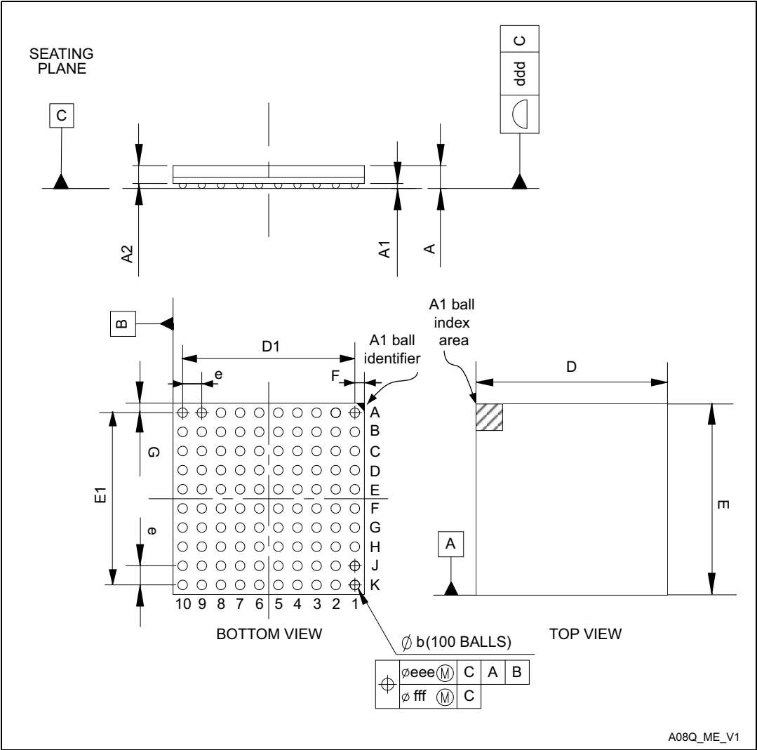
Figure 75. TFBGA100 - Outline
