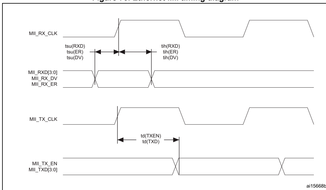
Figure 70. Ethernet MII timing diagram
