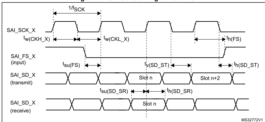
Figure 62. SAI slave timing waveforms
