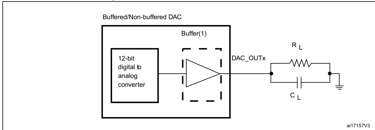
Figure 50. 12-bit buffered /non-buffered DAC
