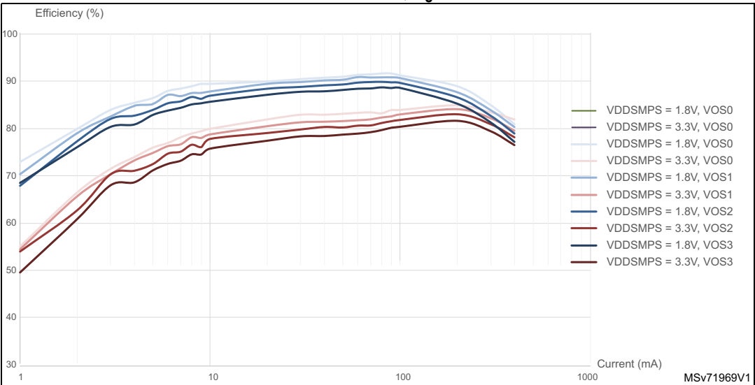
Figure 24. SMPS efficiency versus load current in Run, Sleep and Stop mode with SVOS3 mode, T J = 130 °C
