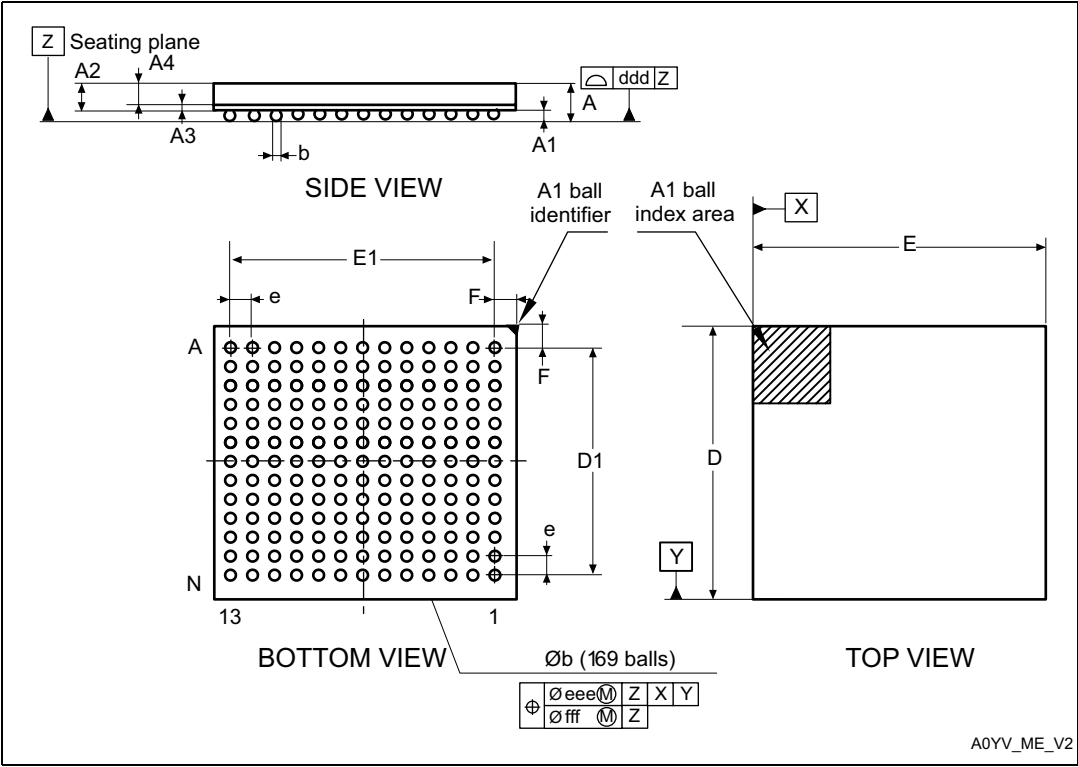
Figure 87. UFBGA169 - Outline
