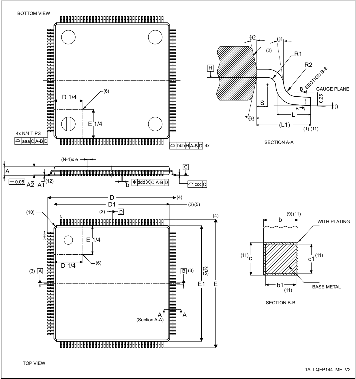
Figure 85. LQFP144 - Outline (15)
