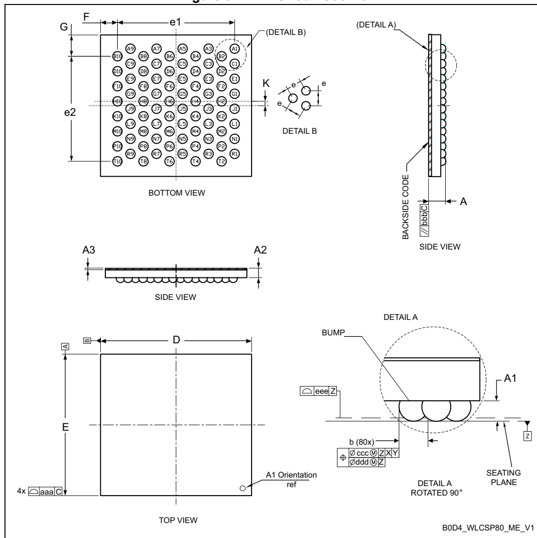
Figure 81. WLCSP80 - Outline
