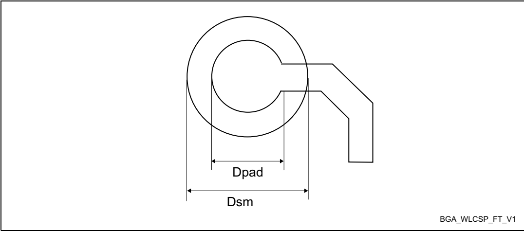
Figure 88. UFBGA169 - Footprint example
