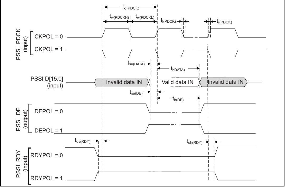
Figure 53. PSSI receive timing diagram
