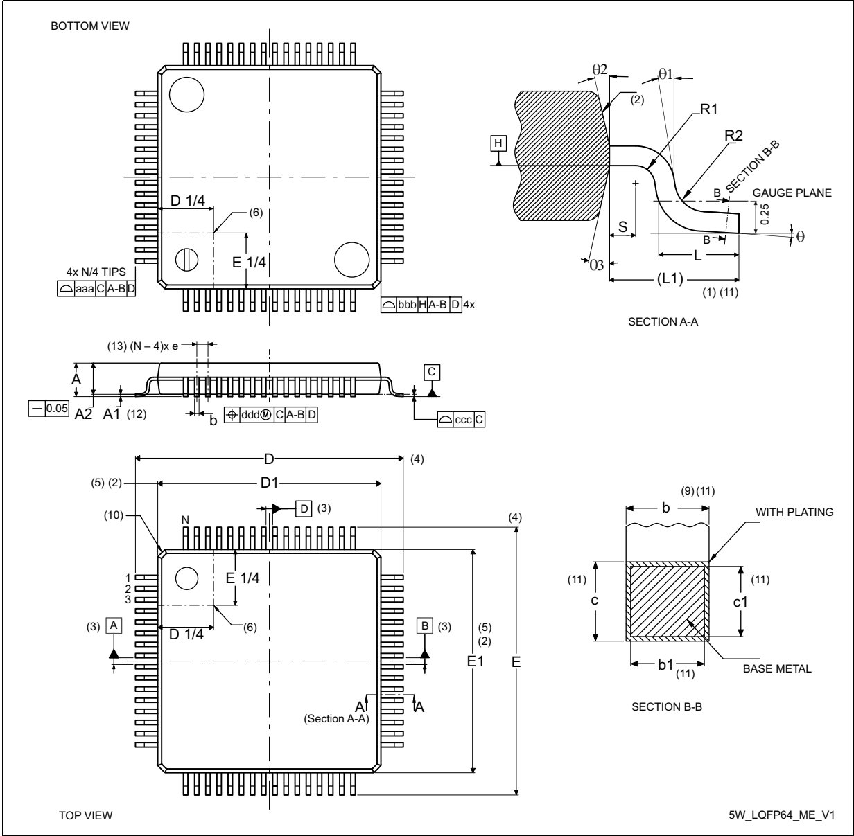
Figure 77. LQFP64 - Outline (15)
