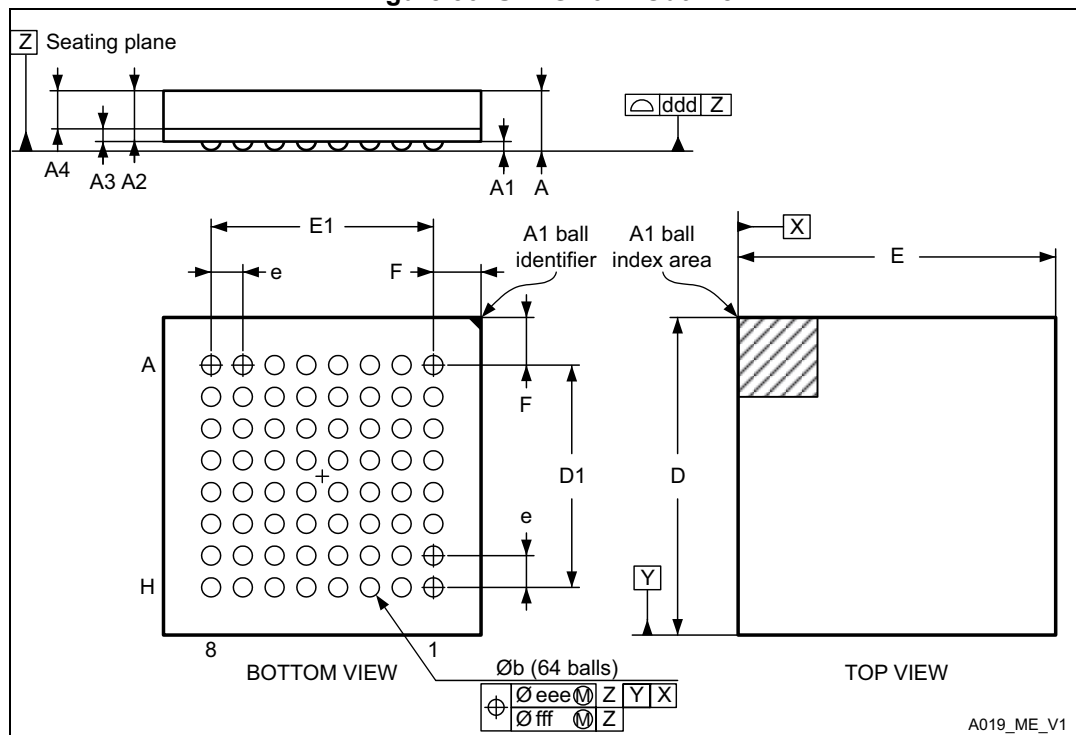
Figure 56. UFBGA64 - Outline
