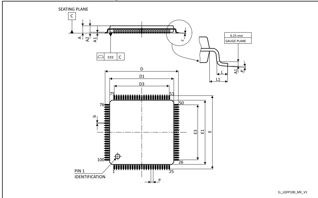
Figure 69. LQFP100 - Outline
