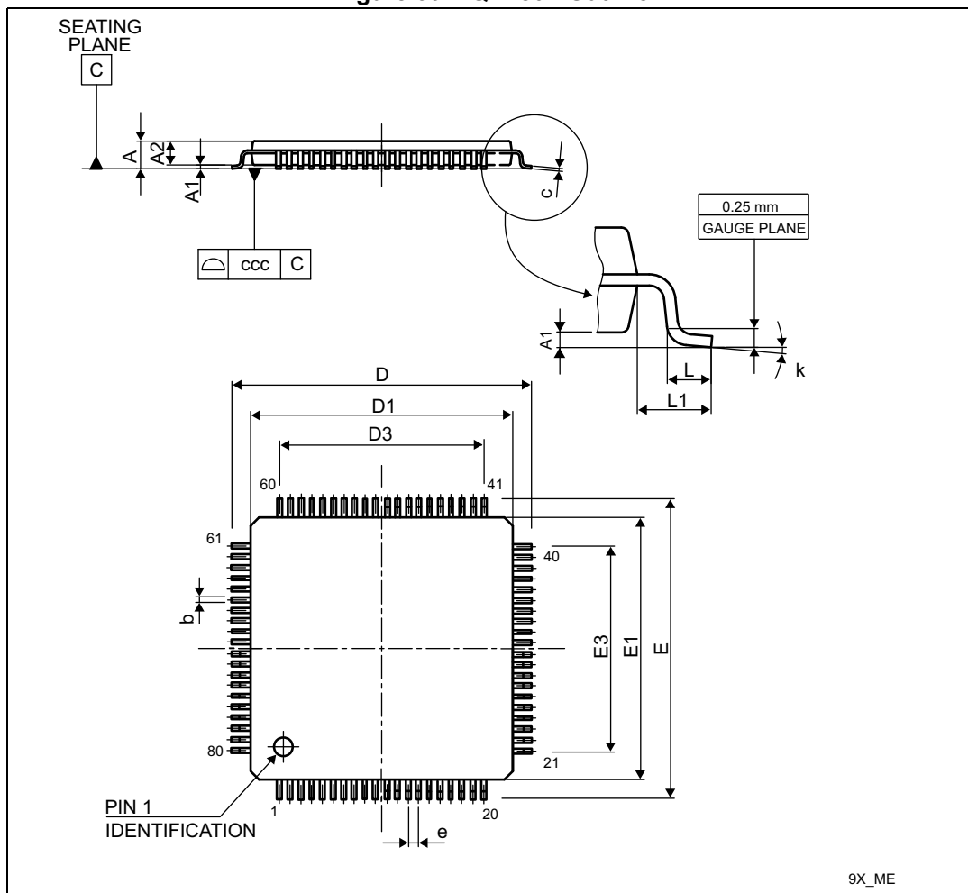
Figure 66. LQFP80 - Outline
