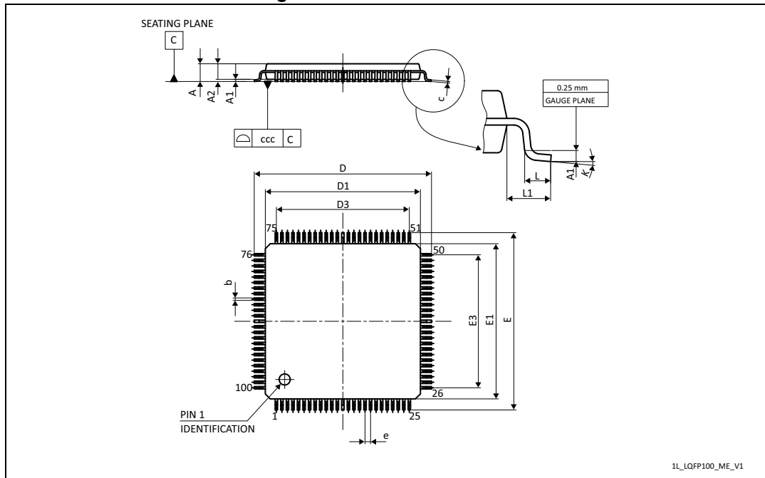
Figure 70. LQFP100 - Outline
