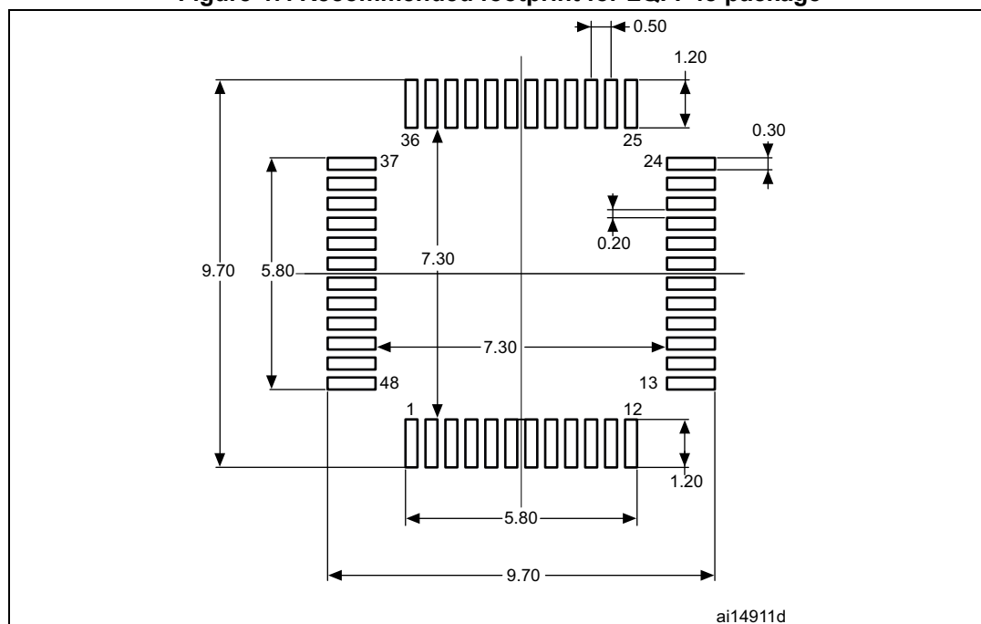
Figure 47. Recommended footprint for LQFP48 package
