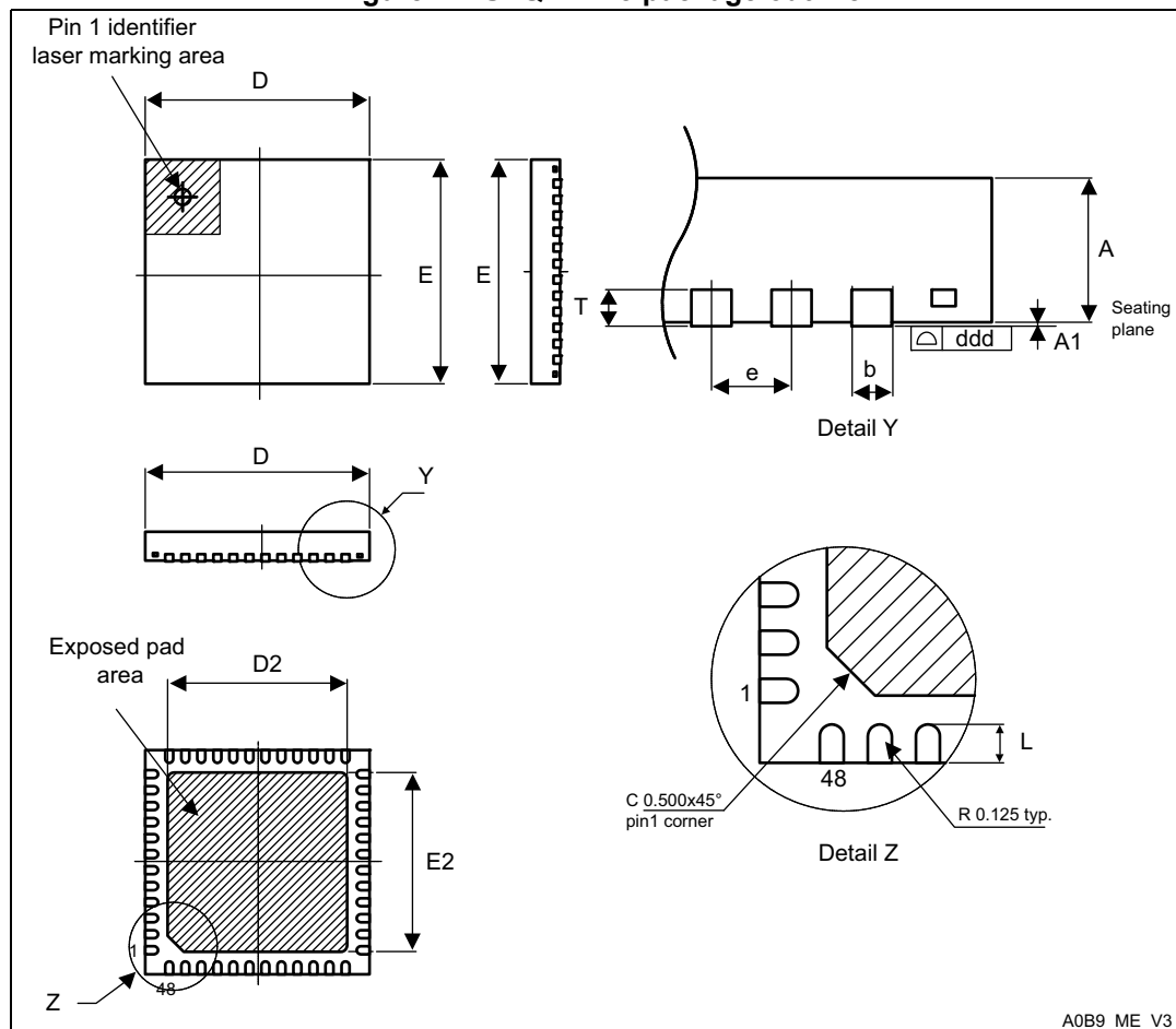
Figure 47. UFQFPN48 package outline
