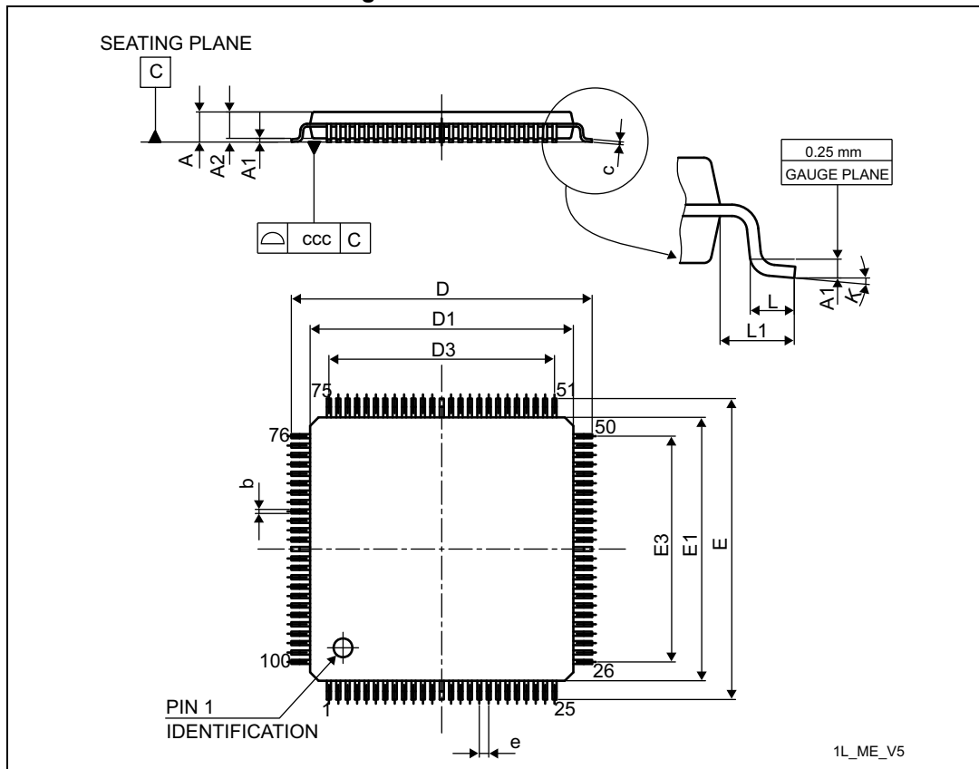
Figure 74. LQFP100 outline
