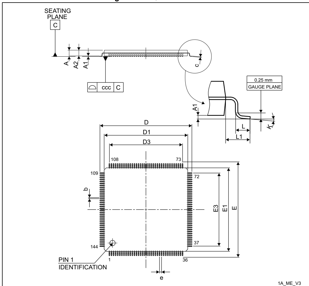
Figure 77. LQFP144 outline
