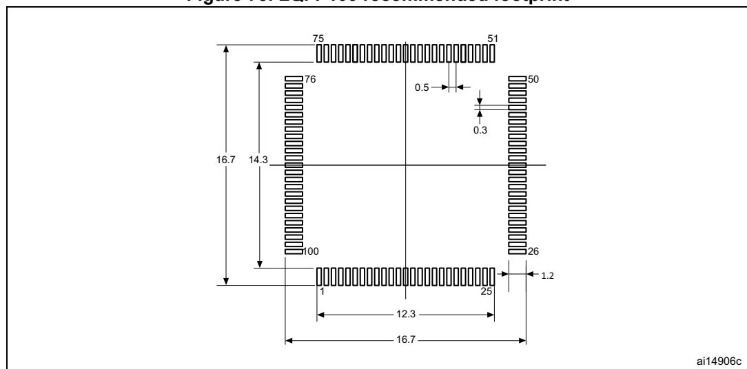
Figure 75. LQFP100 recommended footprint
