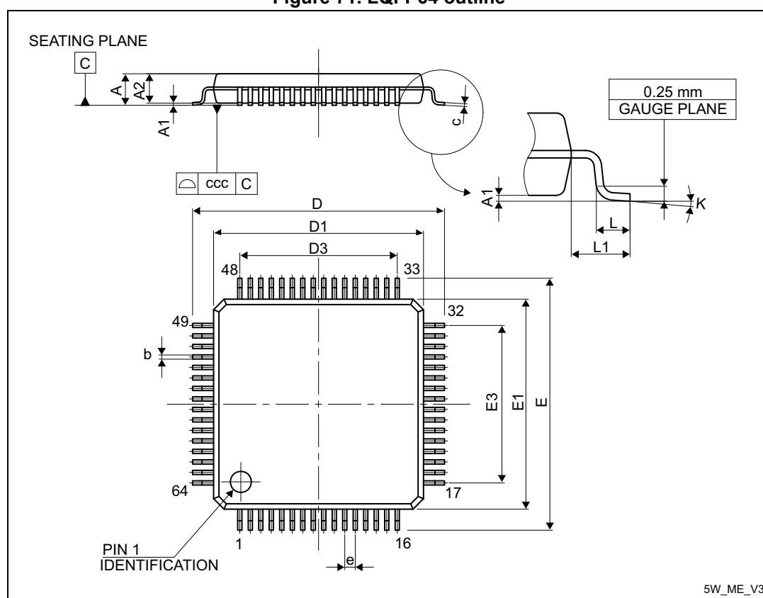
Figure 71. LQFP64 outline
