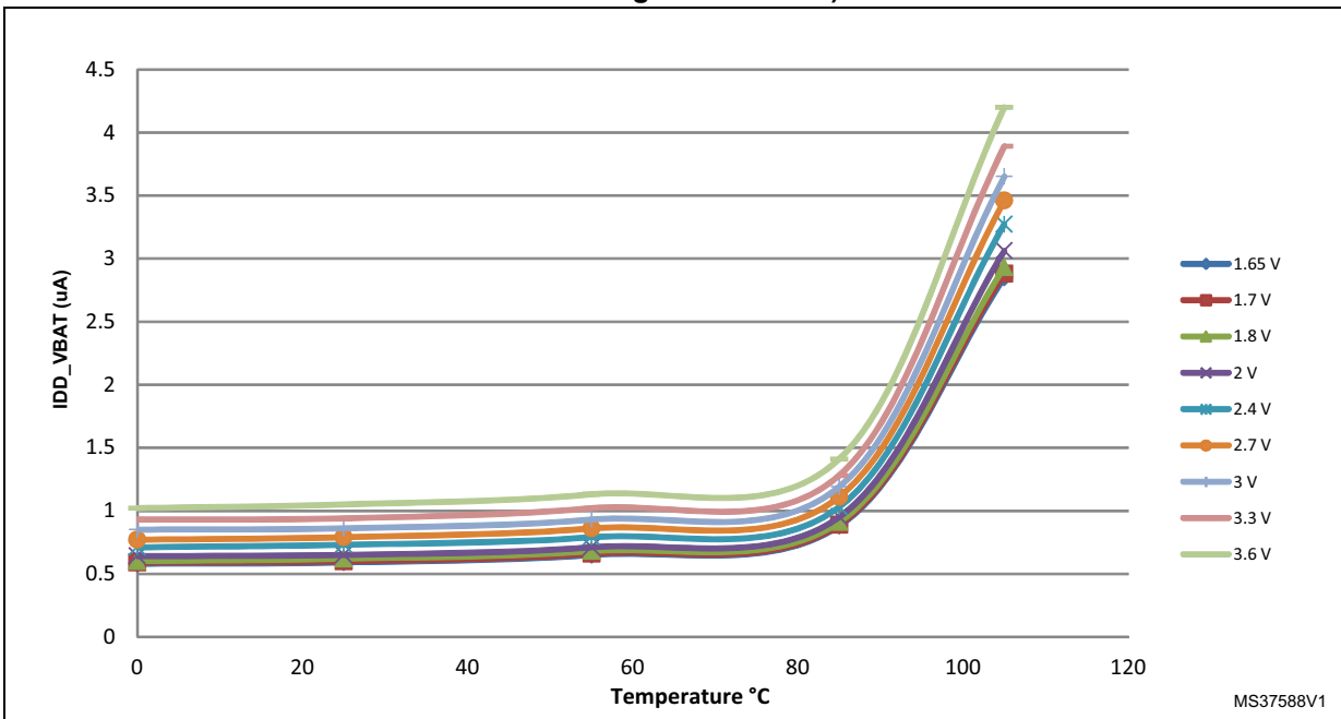
Figure 35. Typical V_{BAT} current consumption (RTC ON/BKP SRAM OFF and LSE in high drive mode)
