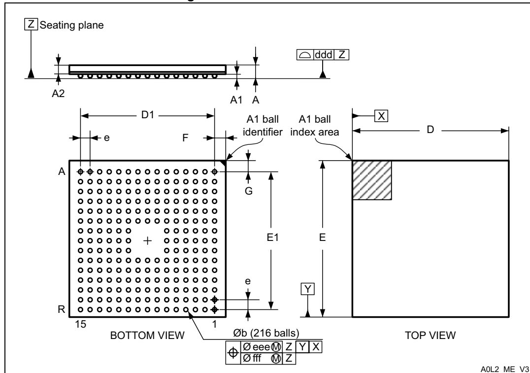
Figure 98. TFBGA216 - Outline
