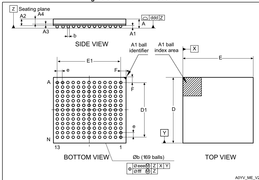
Figure 87. UFBGA169 - Outline
