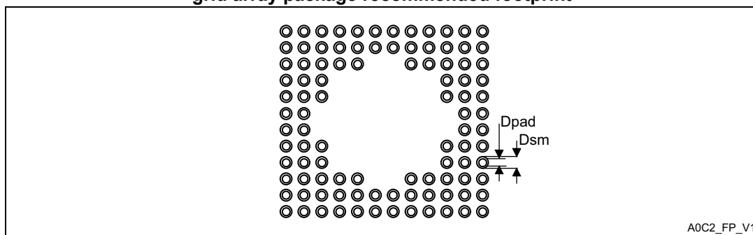
Figure 76. UFBGA100 - 100-pin, 7 x 7 mm, 0.50 mm pitch, ultra fine pitch ball grid array package recommended footprint
