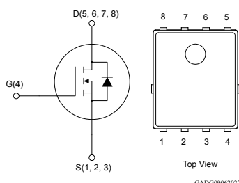
PowerFLAT 5x6
