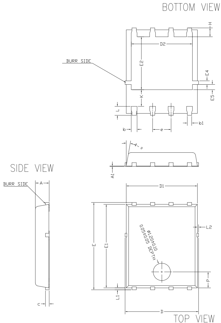
Figure 17. PowerFLAT 5x6 type B package outline
