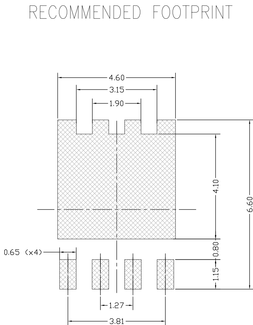
Figure 18. PowerFLAT 5x6 recommended footprint (dimensions are in mm)
