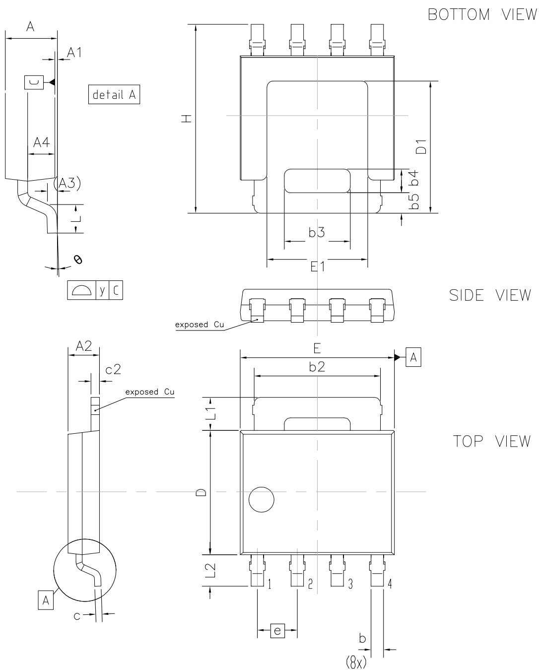
Figure 18. LPAK 5x6 package outline
