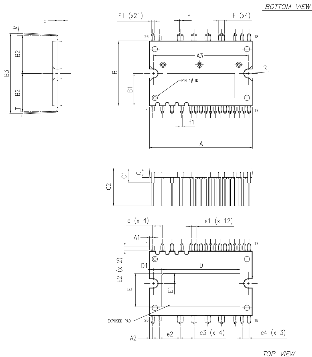
Figure 15. SDIP2B-26L type L3 package outline
