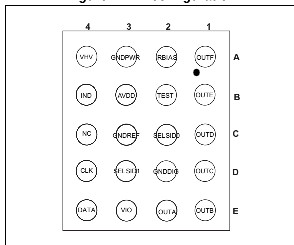
Figure 1. Pin configuration
