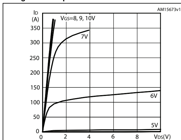
Figure 6. Output characteristics for TO-220
