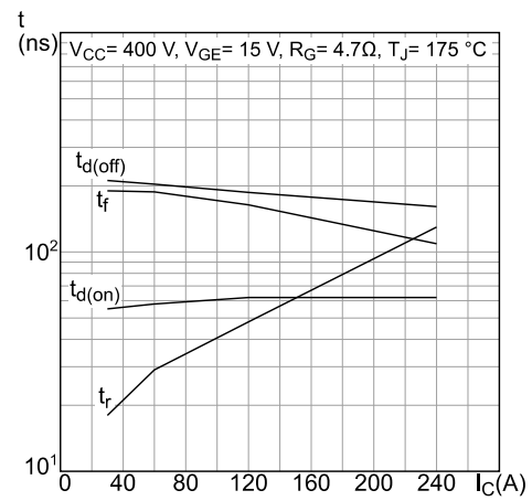
Figure 21: Switching times vs. collector current
