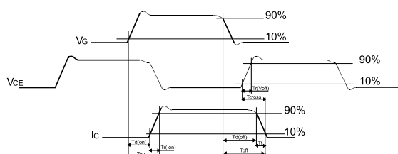
Figure 31: Switching waveform
