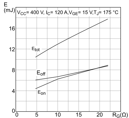
Figure 17: Switching energy vs. gate resistance
