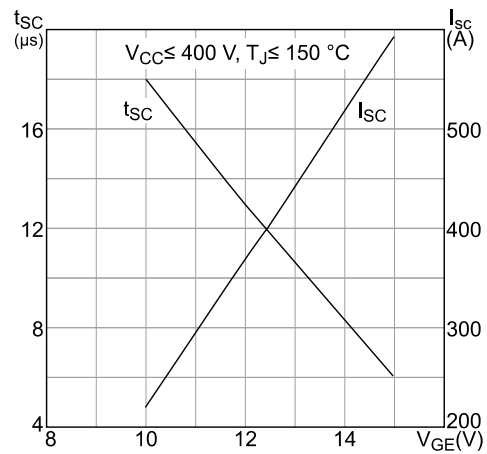
Figure 20: Short circuit time and current vs. V_{GE}
