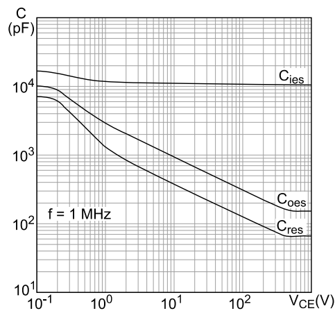
Figure 14: Capacitance variations
