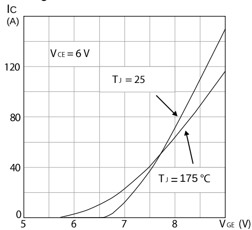
Figure 10: Transfer characteristics
