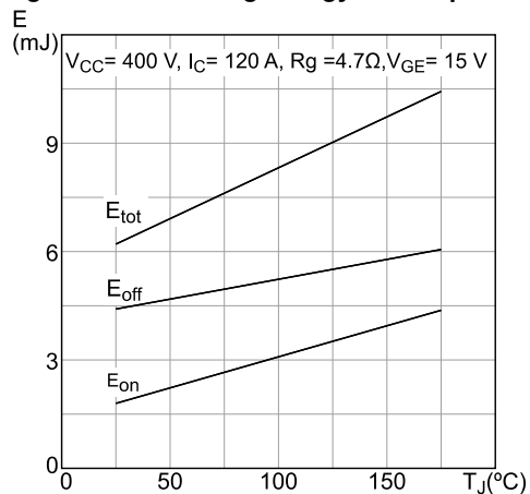
Figure 18: Switching energy vs. temperature
