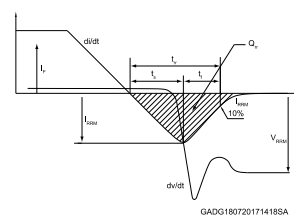
Figure 32: Diode reverse recovery waveform
