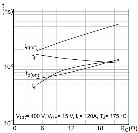
Figure 22: Switching times vs. gate resistance
