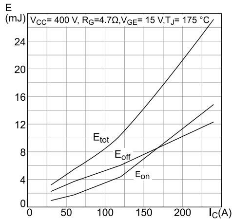
Figure 16: Switching energy vs. collector current
