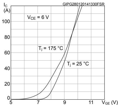
Figure 3. Transfer characteristics
