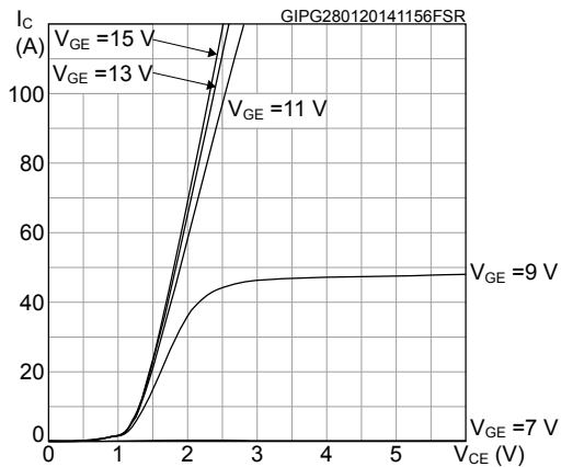
Figure 1. Output characteristics ( T_J = 25^\circ\text{C} )
