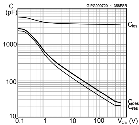
Figure 17. Capacitance variations
