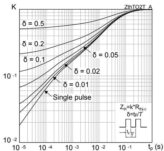
Figure 25. Thermal impedance
