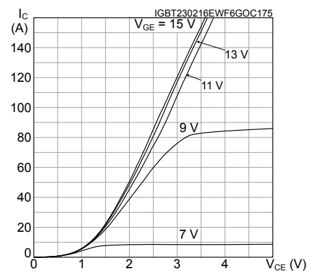
Figure 4. Output characteristics ( T_J = 175^\circ\text{C} )
