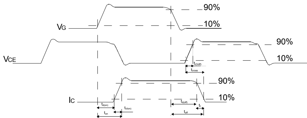
Figure 29. Switching waveform
