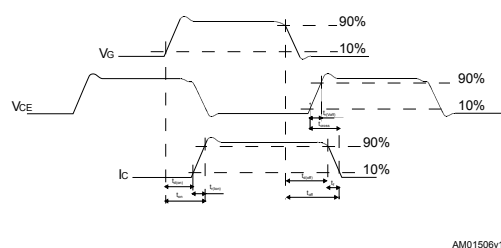
Figure 24. Switching waveform
