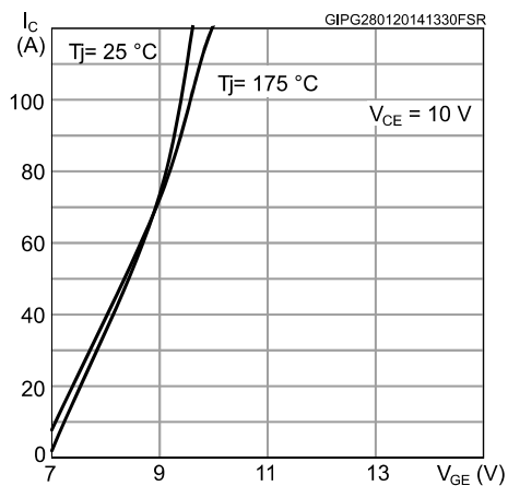
Figure 4: Transfer characteristics
