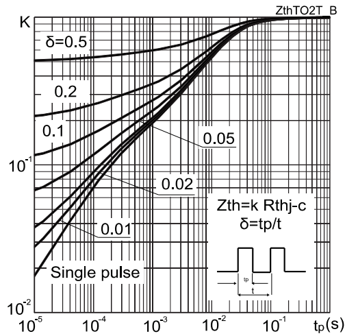
Figure 21: Thermal impedance
