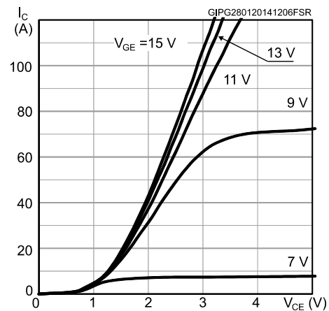
Figure 3: Output characteristics ( T_J = 175^\circ\text{C} )
