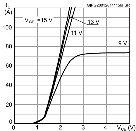
Figure 2: Output characteristics ( T_J = 25^\circ\text{C} )
