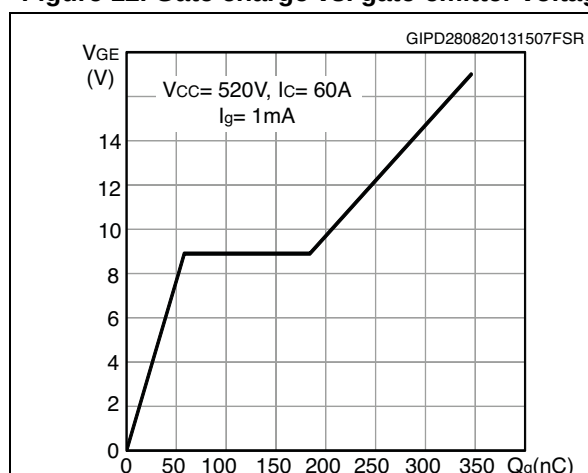
Figure 12. Gate charge vs. gate-emitter voltage
