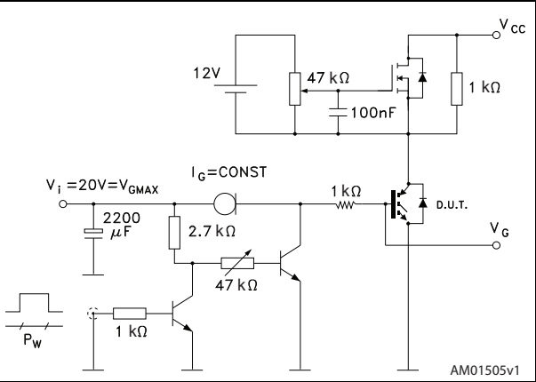
Figure 24. Gate charge test circuit
