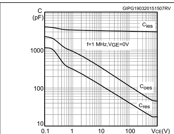
Figure 13. Capacitance variation
