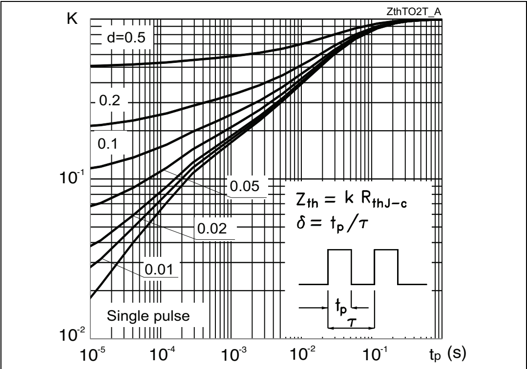
Figure 22. Thermal impedance
