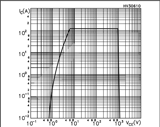
Figure 15. Turn-off SOA
