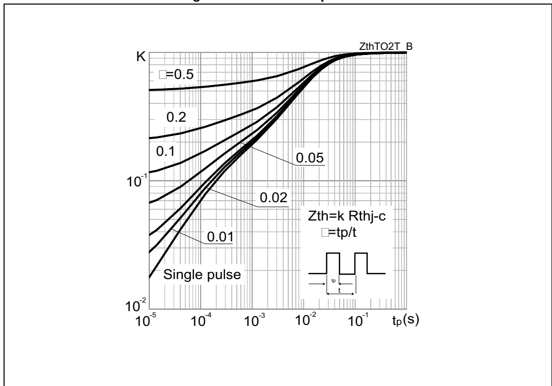
Figure 21. Thermal impedance
