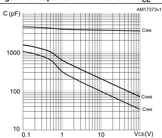
Figure 13. Capacitance variations vs. V_{CE}
