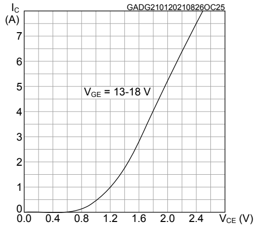
Figure 12. Output characteristics
