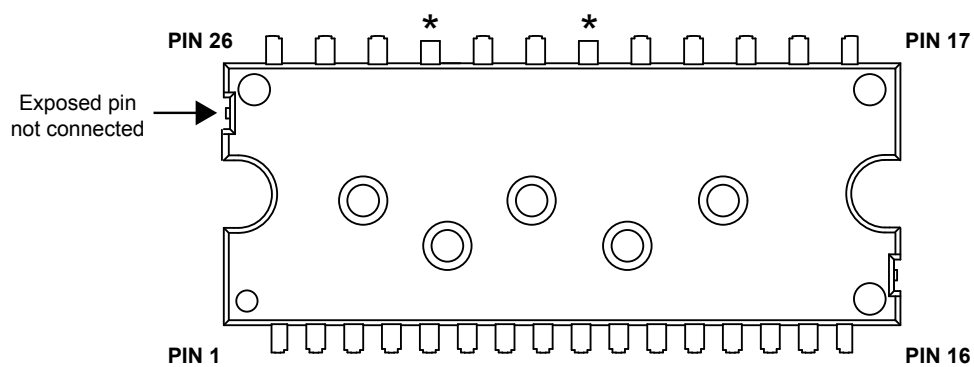
Figure 2. Pin layout (top view) - N2DIP-26L type L
