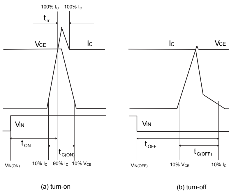
Figure 3. Switching time definition
