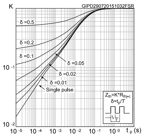
Figure 15. Thermal impedance for IGBT
