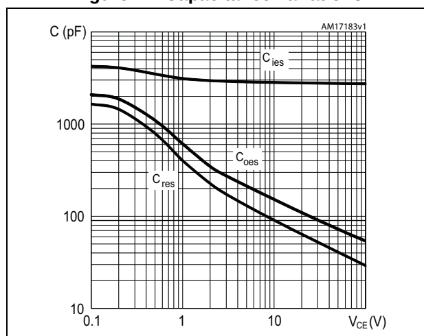
Figure 14. Capacitance variations
