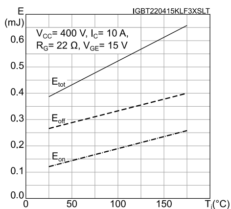
Figure 18: Switching energy vs. temperature
