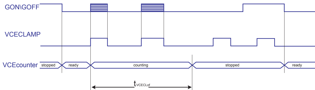
Figure 14. VCECLAMP timing diagram
