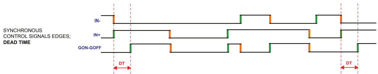
Figure 7. Synchronous control signal edges
