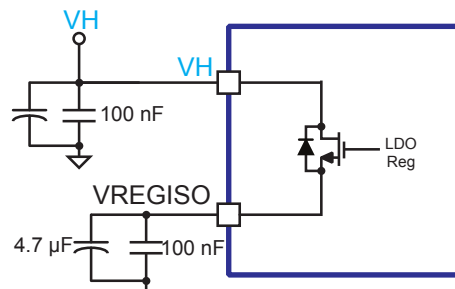
Figure 4. High voltage section 3.3 V voltage regulator
