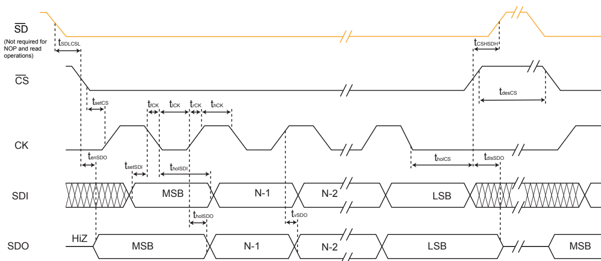
Figure 22. SPI timings
