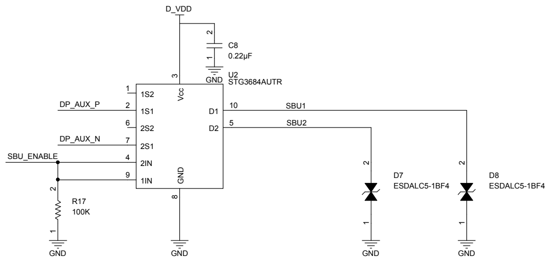
Figure 6. Hi-Speed Data Switch
