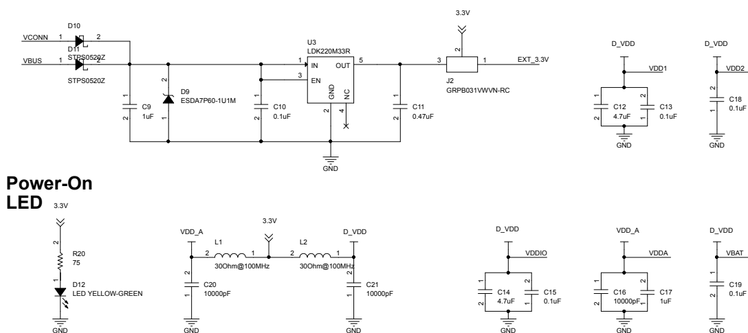
Figure 5. Power Management Stage
